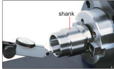
measure radial runout of shank
